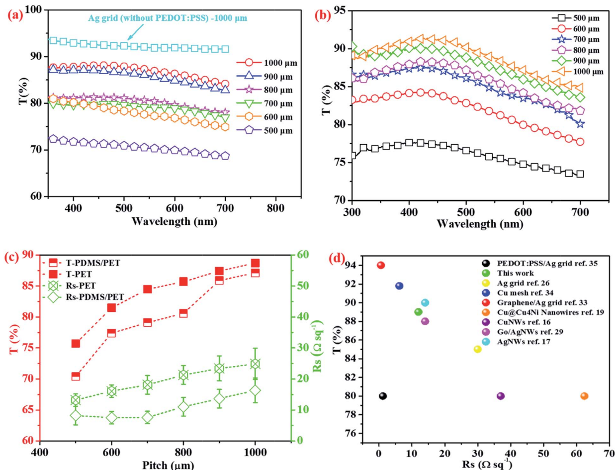
Fig. 2 Optoelectronic performance of PEDOT:PSS/Ag grids on PET and PDMS/PET substrates. (a) The optical transmittance versus wavelength of single Ag grids with pitch of 1000 \mu\text{m} and PEDOT:PSS/Ag grids with various pitches on PET substrate. (b) The optical transmittance versus wavelength of PEDOT:PSS/Ag grids with various pitches on PDMS/PET substrate. (c) The optical transmittance and the sheet resistance versus pitch of PEDOT:PSS/Ag grids on PET and PDMS/PET substrates. (d) The optoelectronic performance of the resultant PEDOT:PSS/Ag grids compared with some other best-performing transparent electrodes previously reported.
